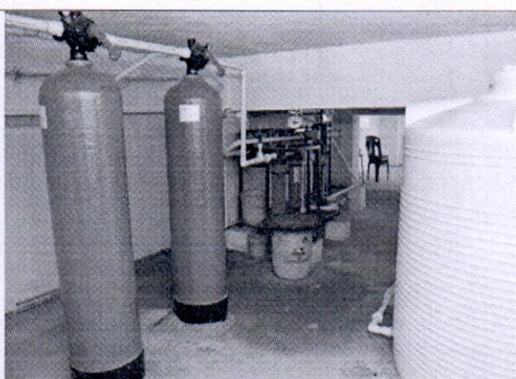
Drinking Water Purification System in the water plant - VFSTR
